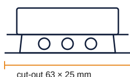
cut-out 63 × 25 mm
