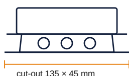
cut-out 135 × 45 mm
