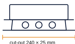
cut-out 240 × 25 mm
