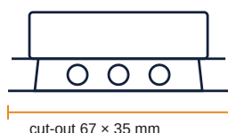
cut-out 67 × 35 mm
