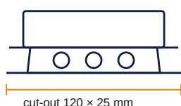
cut-out 120 × 25 mm
