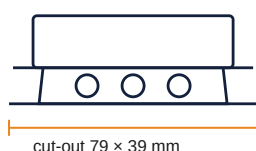
cut-out 79 × 39 mm
