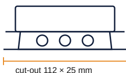
cut-out 112 × 25 mm
